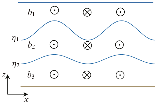
Snapshot of eddying flow
