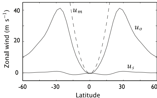
Zonally symmetric
