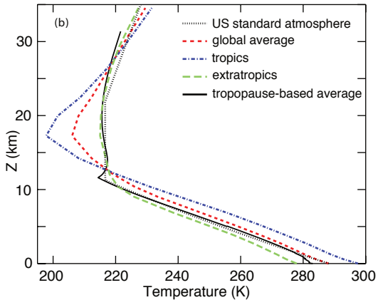
Observed profiles.
