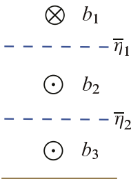
Residual, or thickness-weighted averaged flow
