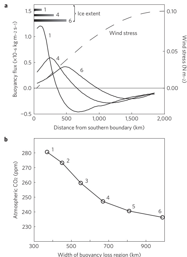
Figure 2 | Forcings and results from the numerical model described in the text and Methods. a , Buoyancy fluxes, ice coverage and wind stress across the southern channel. Solid lines show modern, glacial and an intermediate distribution of buoyancy flux (positive values are buoyancy loss). Ice extent is shown at the top, with fractional coverage shown by depth of shading. Numbers refer to the points in b . The same wind stress (dashed line) is used throughout. b , Steady-state atmospheric CO 2 for buoyancy forcings going from (1) modern to (6) glacial. Changes in CO 2 are those due solely to overturning circulation changes; in practice the implied lower surface temperatures would further enhance the CO 2 reduction in the glacial simulations.
