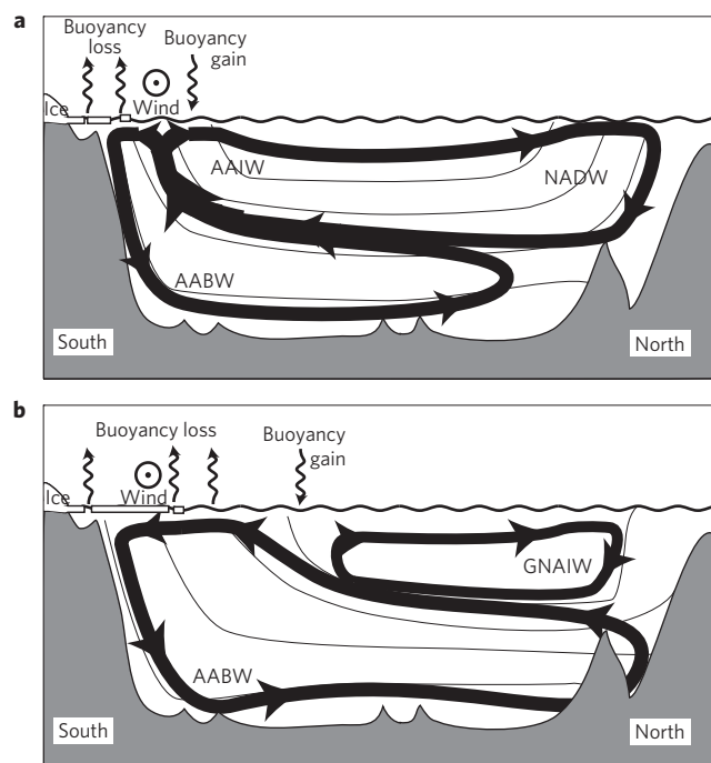
Figure 1 | Schematic of the global overturning with emphasis on the Southern Ocean, in the present day and at the LGM. Thin lines represent density surfaces. a , Modern ocean: NADW and AABW upwell in the Southern Ocean under the influence of the wind. At the surface, southward eddy fluxes dominate where there is surface buoyancy loss, and northward Ekman flux dominates where there is buoyancy gain. b , LGM: a broader region of buoyancy loss gives upwelling at greater distance from the Antarctic continent, farther from the region of AABW formation. Glacial North Atlantic Intermediate Water (GNAIW) is sufficiently light that there is no isopycnal pathway allowing it to return to the surface in the Southern Ocean.
