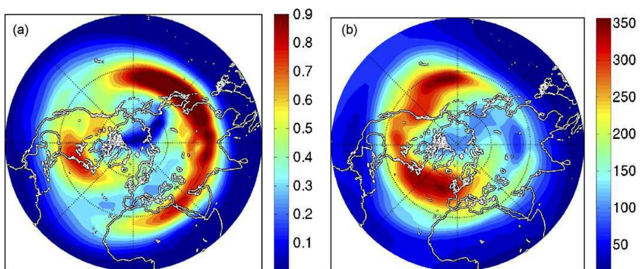
Fig. 2. Left: the Eady growth rate, \sigma_E , at 500 hPa in units of 1/days. Right: The average eddy kinetic energy at 250 hPa in units of (\text{m/s})^2 . Both are for the Northern Hemisphere winter (DJF), computed from the NCEP/NCAR re-analysis. The maxima in EKE are downstream of the maxima in growth rate, and the Pacific storm track does not fully decay before the beginning of the Atlantic storm track. The prime meridian (Greenwich) is at 6 O'clock.
