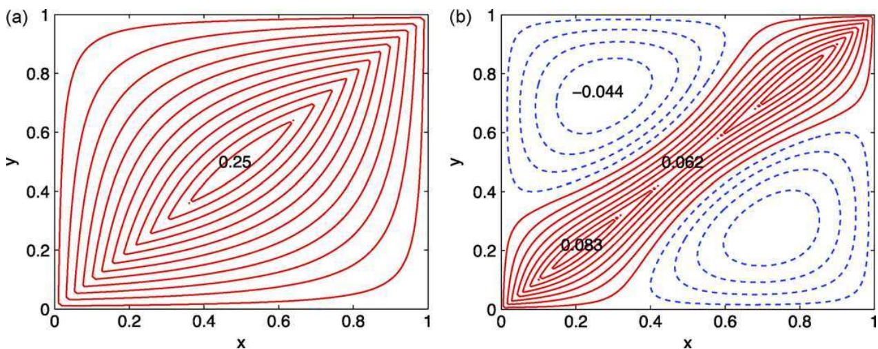
Fig. 8. Covariance function of Brownian bridge (a) and of mean-zero Brownian bridge (b). A given point (x, y) gives the covariance between the two points. The auto-covariance at each point is obtained by traversing the diagonal line from (0,0) to (1,1) . The covariance between a given latitude and all other latitudes is given by taking a horizontal or vertical slice at the chosen latitude.
