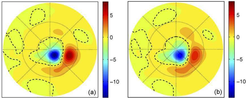
Fig. 15. Teleconnection pattern (hPa) of the two points that have maximum anti-correlation (the two points connected by the white line in panel (b) of Fig. 14). The left pattern uses daily values of surface pressure, and the right panel uses pressure that has undergone a 30 day, low-pass filter. The data are from numerical simulations TM1, as in Figs. 13 and 14b.
