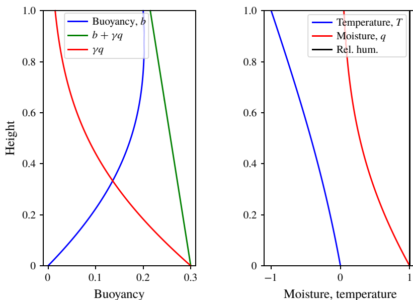
FIGURE 1. (Colour online) A non-dimensional drizzle solution with saturated upper and lower boundaries. The boundary conditions are that b = 0 at z = 0 and b = 0.2 at z = 1 and q = q_s at both boundaries, thus giving the values of m (= b + \gamma q) at the boundaries shown. These solutions were obtained with \gamma = 0.3 , \alpha = 3 and \beta = 1.2 .
