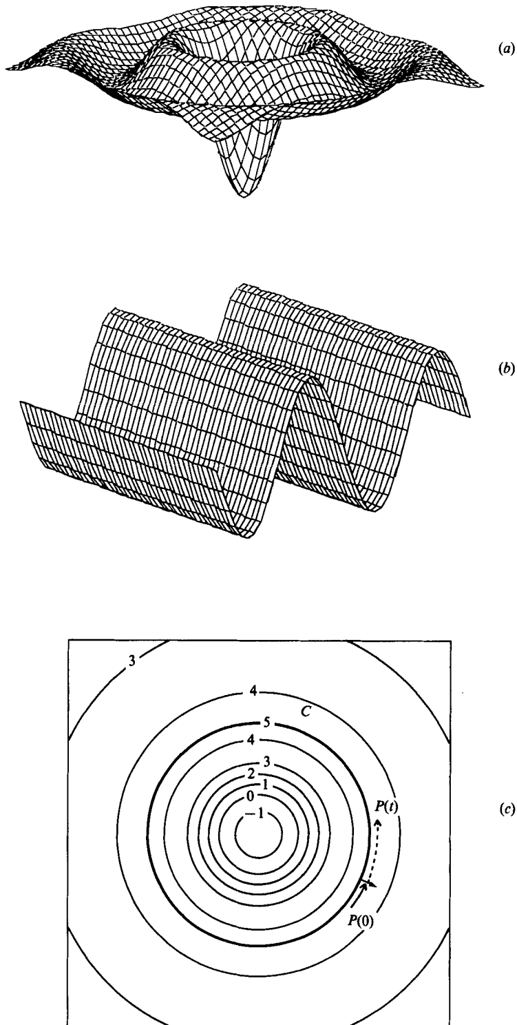
FIGURE 2. (a, b) Idealized three-dimensional plots of energy on a sheet. In both cases energy maxima exist that are not stable. (c) Contour plot of case (a). The growth of a perturbation P off the energy maximum contour C is not bounded by its initial size.
