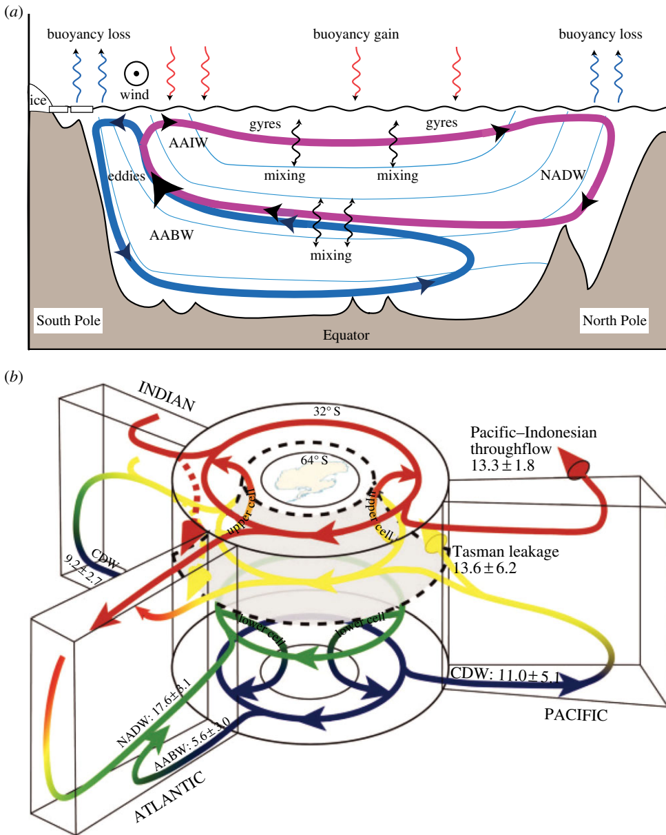
Figure 7. Two views of the meridional overturning circulation, not to scale. (a) The MOC in a single basin resembling the Atlantic, and which is now reasonably well understood with a combination of idealized and comprehensive models and observations. GFD has yet to fully come to grips with the more complex, multi-basin reality (b) (courtesy of K. Speer), although it may yet be a minor extension of the single-basin picture. AABW, Antarctic Bottom Water; AAIW, Antarctic Intermediate Water; CDW, Circumpolar Deep Water; NADW, North Atlantic Deep Water. (Online version in colour.)
