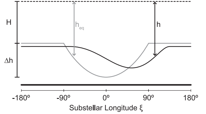
Figure 1. Equilibrium profile h_{eq} represents the heating effect as a thickening of the geopotential of the upper atmosphere. Where the stellar insolation irradiates the dayside of the planet, the geopotential gh is forced toward a deeper equilibrium depth. The rate at which the geopotential is forced toward the equilibrium profile is determined by the radiative cooling timescale \tau_{rad} .
