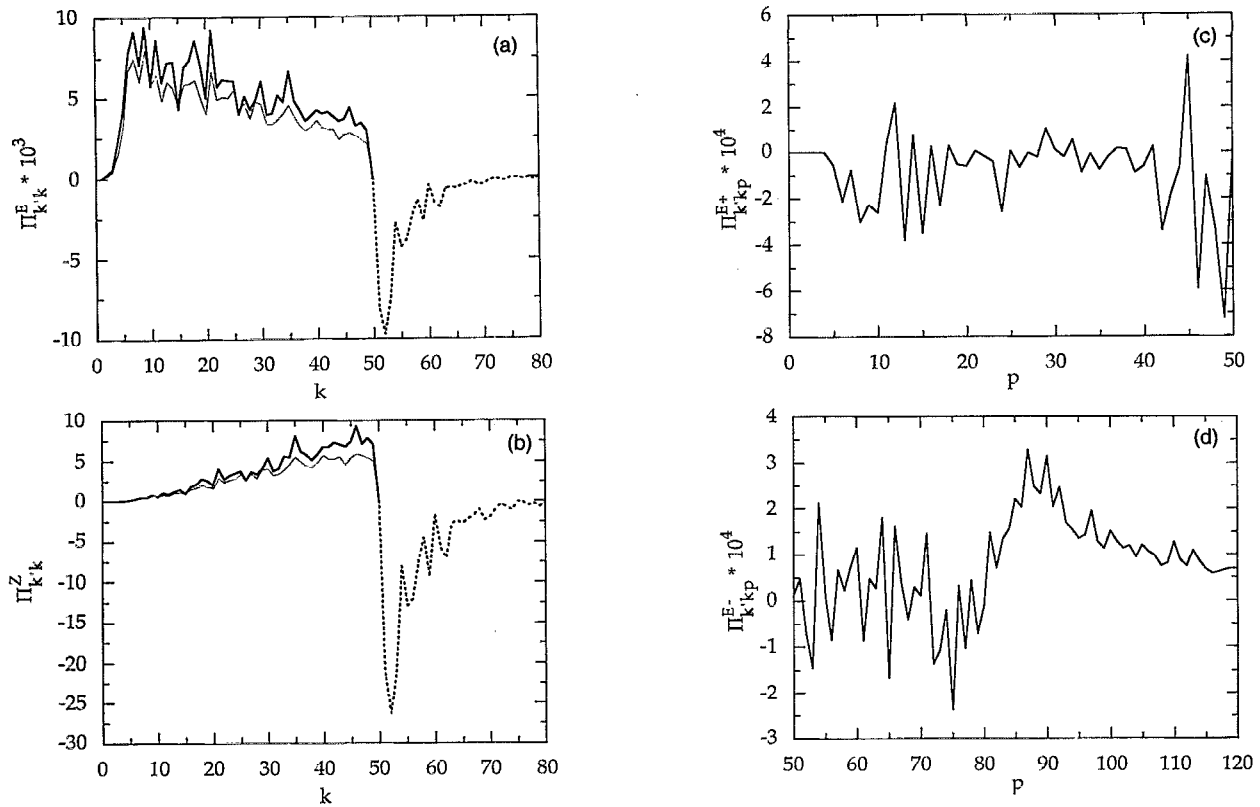
FIG. 13. Contributions to the energy inertial range flux for k'=50 . (a) The energy flux contributions \Pi_{k'k}^{E+} (dashed curve) and \Pi_{k'k}^{E-} (thick solid curve). The thin solid curve is the contribution to \Pi_{k'k}^{E-} for p > k_f , where k_f=80 defines the lower end of the forcing range. (b) The enstrophy flux contributions \Pi_{k'k}^{Z+} (dashed curve) and \Pi_{k'k}^{Z-} (thick solid curve). The thin solid curve has the same meaning as in (a). (c) The p dependence of \Pi_{k'k}^{E+} for k=55 . (d) The p dependence of \Pi_{k'k}^{E-} for k=10 .
