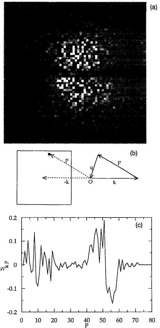
FIG. 3. (a) The time-averaged enstrophy transfer function S_{kp} for \mathbf{k}=(50,0) . Areas blacker than the background gray have positive values of S_{kp} , with solid black denoting the highest value; similarly, white denotes negative values. The plot is centered (in \mathbf{p} space) at \mathbf{p}=-\mathbf{k} . (b) Schematic for interpreting (a). Given the triangle made of solid vectors ( \mathbf{k}+\mathbf{p}+\mathbf{q}=0 ), the dashed vectors represent their orientation in the plot of S_{kp} . The square outline denotes the border of (a) above and "O" is the origin ( p_x, p_y ) = (0,0). The small black square at the end of the dashed \mathbf{p} vector represents an S_{kp} grid point. (c) S_{kp} from a averaged over angle in \mathbf{p} space.
