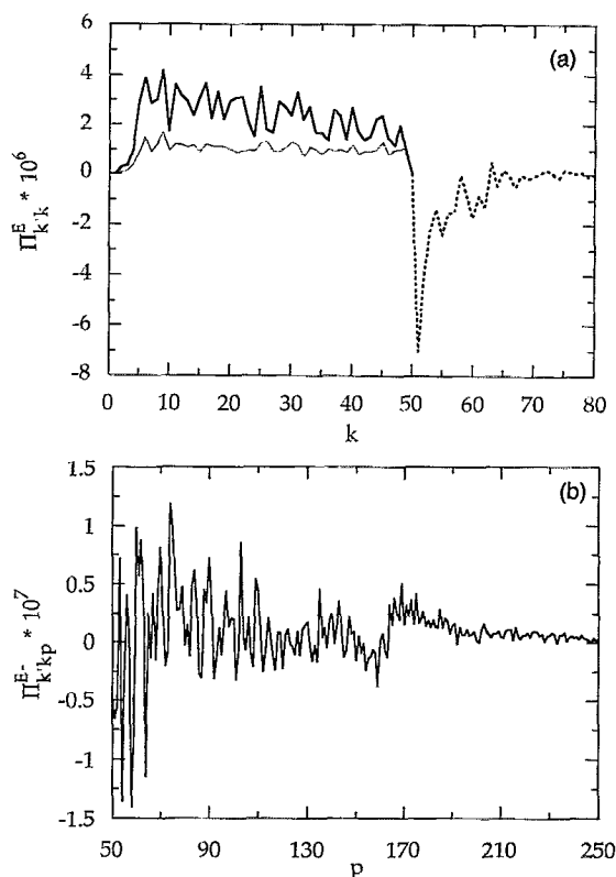
FIG. 14. Contributions to the energy inertial range flux for k'=50 from a high resolution run with forcing in the range 160 < k < 165 . (a) \Pi_{k'k}^{E+} (dashed curve) and \Pi_{k'k}^{E-} (thick solid curve). The thin solid curve is the contribution to \Pi_{k'k}^{E-} for p > k_f , where k_f=160 defines the lower end of the forcing range. (b) The p dependence of \Pi_{k'kp}^{E-} for k=10 .
