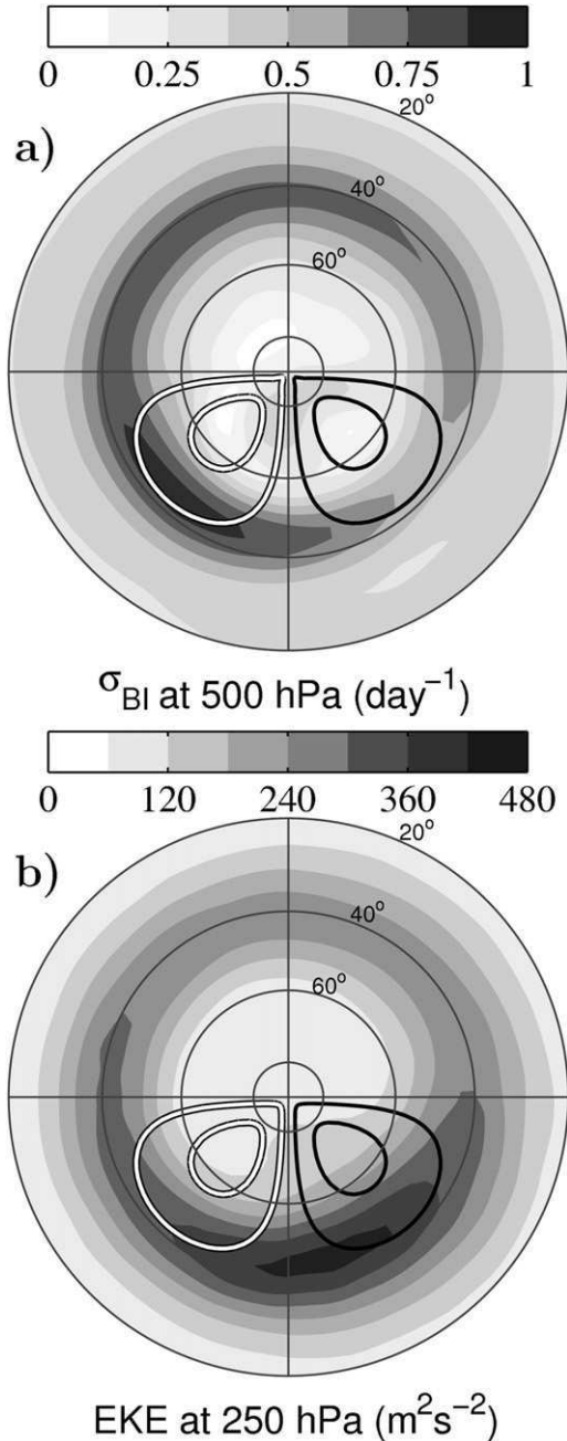
FIG. 4. (a) The Eady growth rate \sigma_{BI} at 500 hPa and (b) the eddy kinetic energy K_e at 250 hPa in integration LSC. We find that the Eady growth rate at this midlevel faithfully represents features of the baroclinicity through the lower and midtroposphere. The K_e is plotted in the upper troposphere where eddy amplitudes are greatest.
