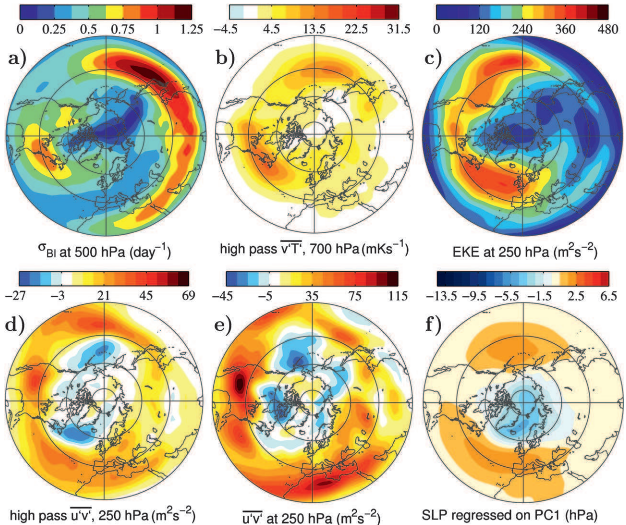
FIG. 10. Evidence of the eddy life cycle in the NH boreal winter (DJF) climatology and its relationship to the NAM. (a) The midtropospheric Eady growth rate, (b) lower-troposphere 2–10-day high-pass eddy heat fluxes, (c) upper-tropospheric kinetic energy, (d) high-pass eddy momentum fluxes, (e) total eddy momentum fluxes, and (f) NAM loading pattern, expressed as an anomaly of SLP. The Eady growth rate \sigma_{BI} was computed from the winter average climatology at 500 hPa. The eddy heat flux \overline{v'T'} was computed at 700 hPa, and the EKE and momentum fluxes \overline{u'v'} at 250 hPa. The NAM pattern was computed by regressing the daily SLP anomalies on the standardized NAM index. The color scale is the same as that used in the respective plots based on our model integrations.
