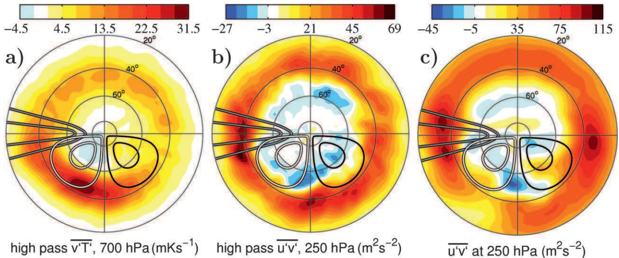
FIG. 8. (a) The 2–10-day eddy heat fluxes, (b) the 2–10-day eddy momentum fluxes, and (c) the total eddy momentum fluxes for integration LSC+RM. The eddy heat flux \overline{v'T'} was computed at 700 hPa, and the momentum flux \overline{u'v'} at 250 hPa.
