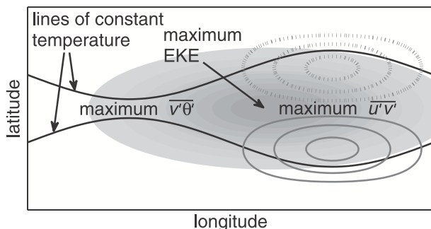
FIG. 14. A diagram illustrating the relationship between intra-seasonal variability (the dipole pattern shown with solid and dashed gray contours), the baroclinicity of the flow (as inferred from the black contours of temperature), and the eddy statistics. Eddy growth dominates in the baroclinic regions, but eddies continue to grow as they are advected downstream. Downstream development tends to maintain the eddy kinetic energy despite variation in the growth rates. Most critical is a diffluent region in which the weak upper-level flow cannot support as many waves and wave breaking and dissipation begin to dominate, producing eddy momentum fluxes. Intraseasonal variability is the response to this stirring of the large-scale flow by eddies.
