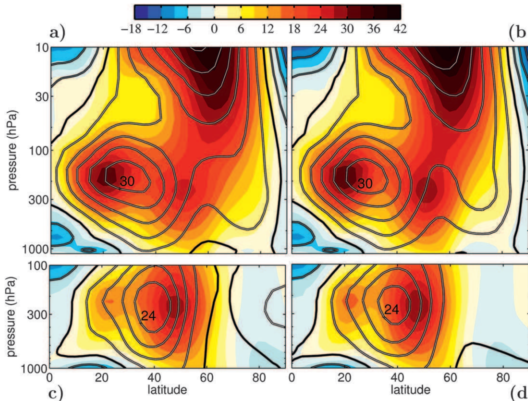
FIG. 13. Jet composites of the zonal winds based on (a),(c) the NAM index and (b),(d) jet separation analysis. We find that the jet separation analysis provides the same information as composites based on the NAM index for both the (a),(b) reanalyses and (c),(d) model winds. The contours illustrate composites based on cases in which the NAM index is low on the left and in which there is just one distinct jet on the right. Shading illustrates composites based on times when the NAM index is high on the left and there are two well-separated jets on the right. The winds are averaged in just the quadrant with peak NAM/NAO loading: between 70°W and 20°E for reanalyses and between 0° and 90°E for model output.
