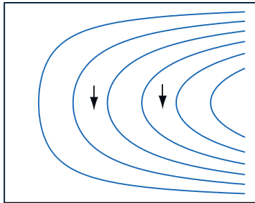
Eastern boundary layer
