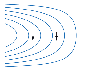
Western boundary layer
