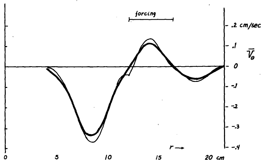
FIG. 7. Computed mean zonal flow \bar{V}_\theta as for Fig. 6. The thin line is unsmoothed, the thick line smoothed with a paraboloidal filter of half-width 1.5 cm.
