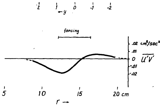
FIG. 1. Measured Reynolds stress \overline{u'v'} = -\overline{V_\theta V_r} vs radius r in a cylinder of radius R = 21.4 cm, initial depth H_0 = 8 cm, rotation rate \Omega = 4.82 s ^{-1} , wavenumber n = 6 , retrograde forcing at n\omega = -0.32 s ^{-1} , and an amplitude W_0 = 0.05 cm s ^{-1} . Half-second streaks of surface particles gave discrete measurements which were smoothed by a paraboloidal weighting filter of half-width 1.5 cm.
