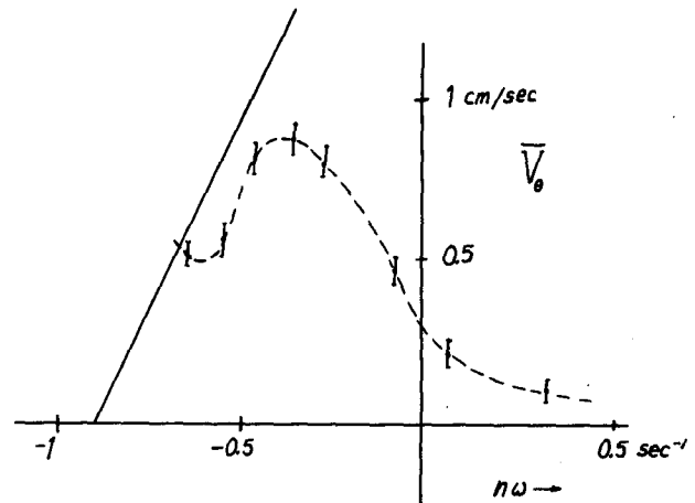
FIG. 3. Measured mean zonal velocity \bar{V}_\theta at r = 14.25 cm radius vs n\omega for forcing with amplitude W_0 = 0.2 cm s ^{-1} in a cylinder of radius R = 21.4 cm, initial depth H_0 = 6 cm, rotation rate \Omega = 4.23 s ^{-1} and wavenumber n = 6 .
