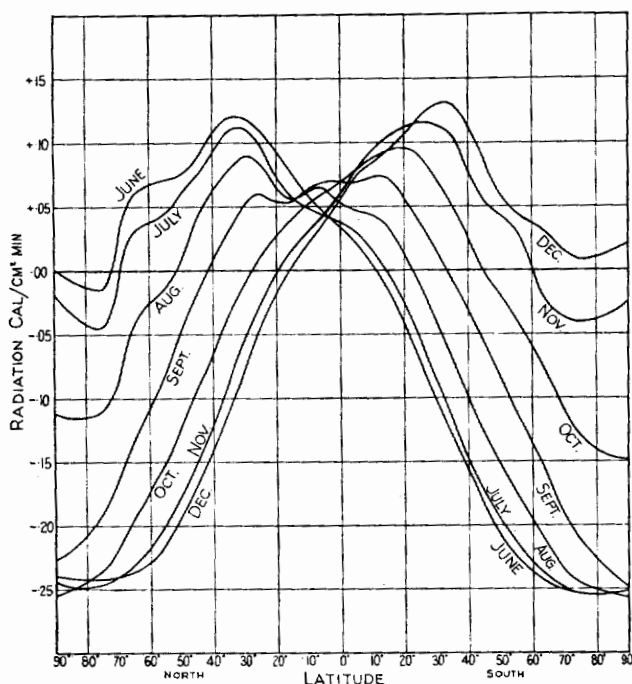
Fig. 12.—Intensity of the net radiation, June to December.
