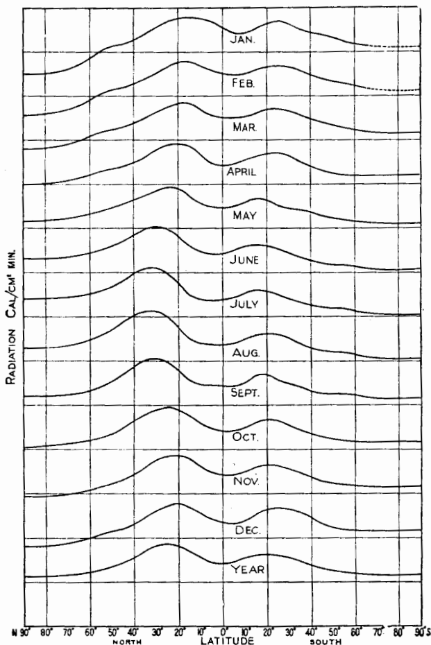
FIG. 10.—Intensity of outgoing terrestrial radiation.
