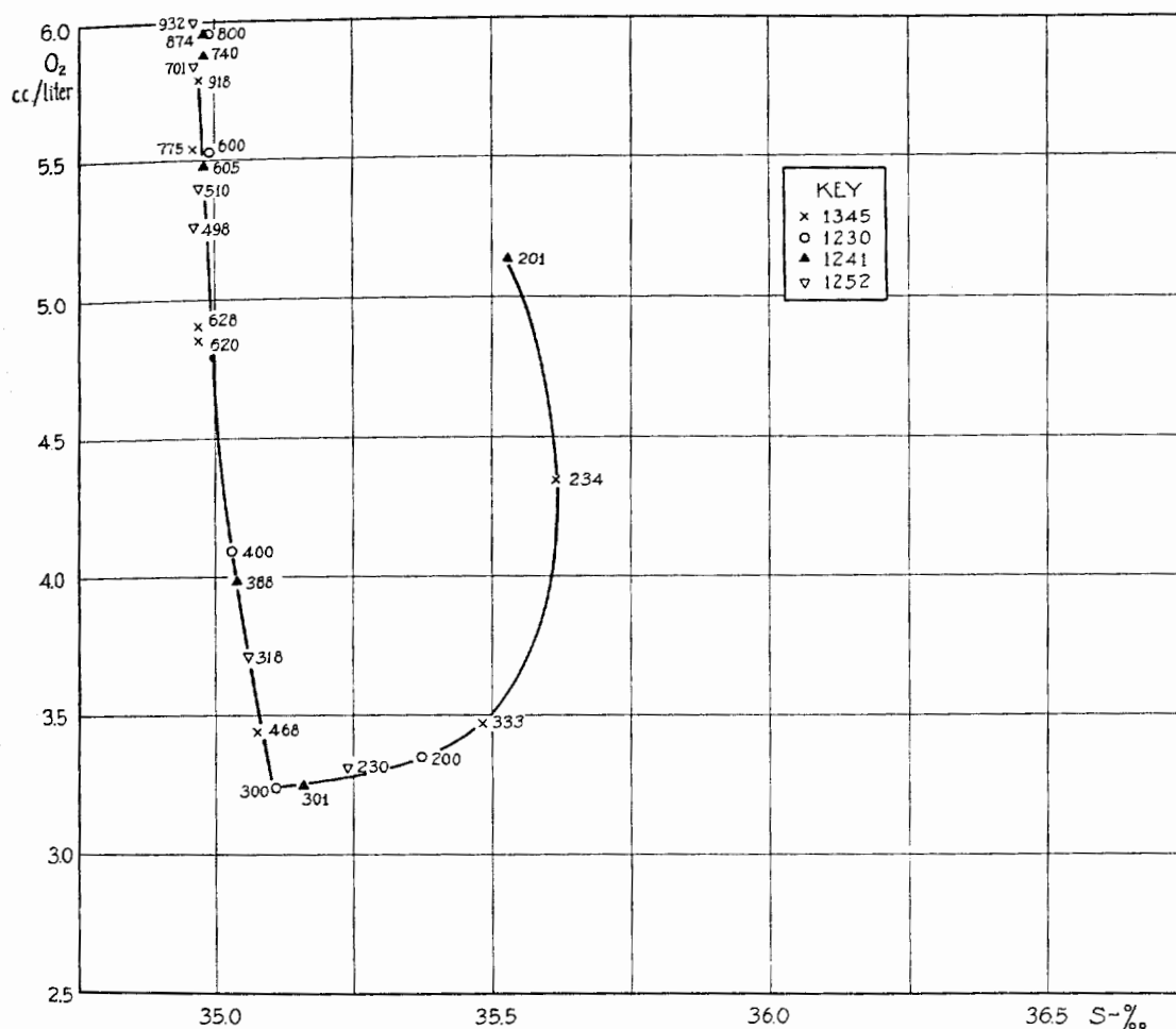
FIG. 20.—Average oxygen-salinity correlation curve for selected slope water stations.
