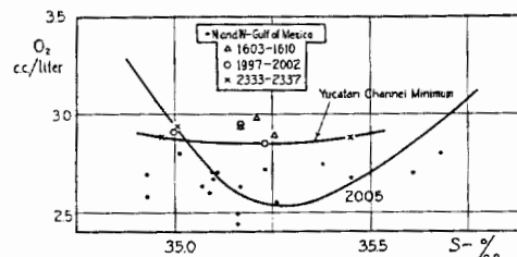
FIG. 16.—Comparison between minimum oxygen content of water passing through the Yucatan Channel and the minimum oxygen content in the Havana section (station 2005) and at stations in the northern and western parts of the Gulf of Mexico.
