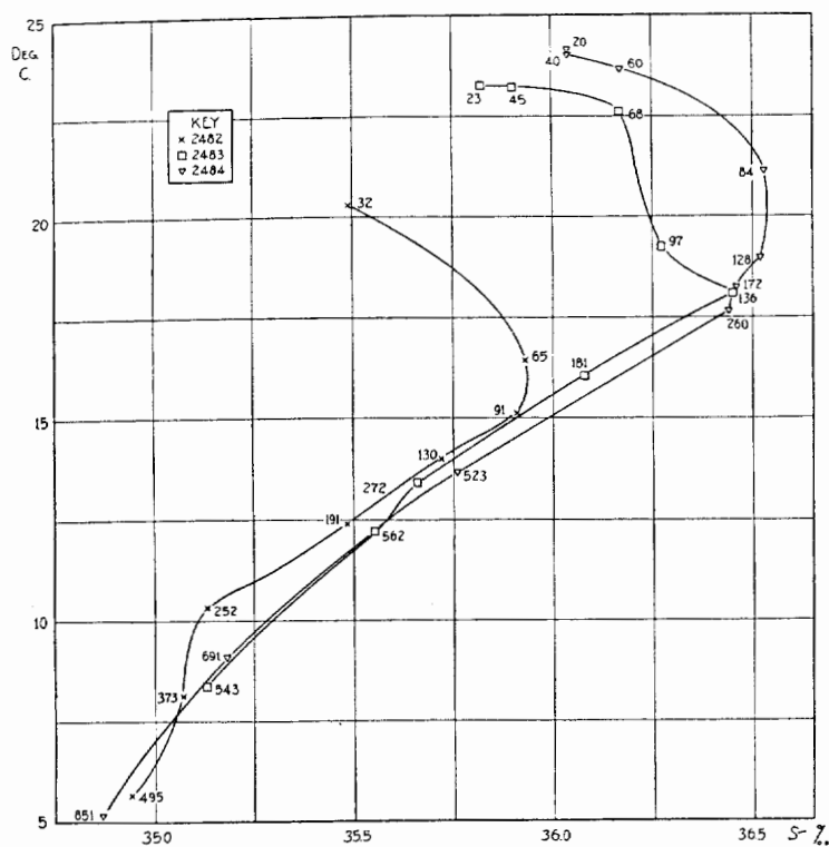
FIG. 13.—Temperature-salinity correlation curves for the Grand Banks section.
