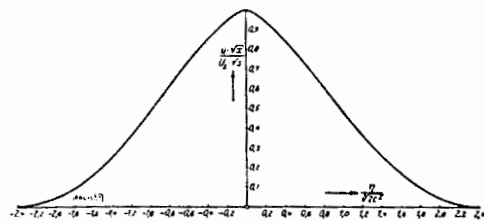
FIG. 2.—Non-dimensional representation of theoretical distribution of axial velocities in two-dimensional wake stream, according to Tollmien.
