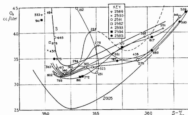
FIG. 23.—Oxygen-salinity correlation curves for the Georges Bank section.
