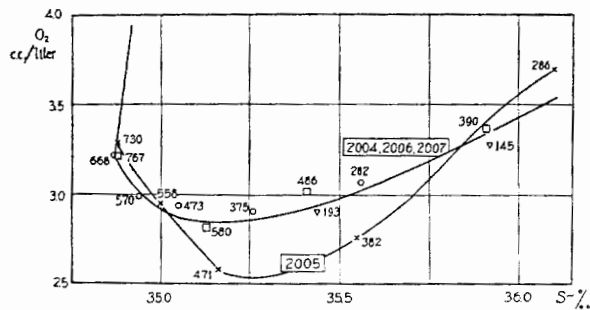
FIG. 17.—Oxygen-salinity correlation curves for the Havana section.
