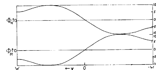
Fig. 3. Graph of the solutions \Phi_{1t} and \Phi_{3t} of the averaged vorticity equations. The scale on the right side shows the corresponding value of the mean height tendency in \text{m day}^{-1} when T_i^* is taken as 0.5^\circ \text{C day}^{-1} .
