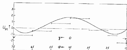
Fig. 5. U_{3t} in \text{m sec}^{-1} \text{ day}^{-1} when T_t^* is taken as 1^\circ \text{C day}^{-1} . The dotted horizontal line segments are the values of \partial U/\partial t computed from Widger's data in table I.
