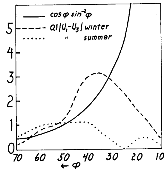
Fig. 2. The satisfaction of the stability criterion for baroclinic waves in the two-level model as a function of latitude and season. The curves of 0.1 (U_1 - U_3) (in \text{m sec}^{-1} ) are taken from the cross sections of HESS.
