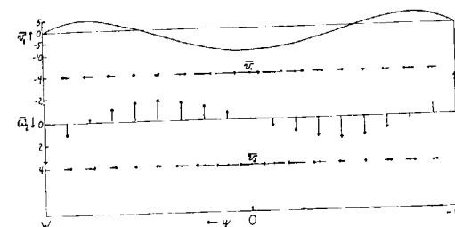
Fig. 4. The meridional circulation due to the baroclinic waves. The arrows indicate the direction and intensity of the flow. Values of \bar{\omega}_2 and \bar{v}_1 when T_i^* is taken as 0.5^\circ \text{C day}^{-1} are indicated by the scales on the left side; \bar{\omega}_2 is in units of \text{mb day}^{-1} and \bar{v}_1 (top line) is in units of \text{cm sec}^{-1} .
