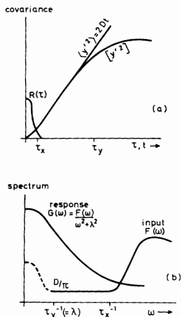
Fig. 2. Input and response of stochastically forced (single component) climate model with linear feedback; (a) covariances, (b) spectra. In the ranges \tau_x \leq \tau \leq \tau_y and \tau_y^{-1} \leq \omega \leq \tau_x^{-1} the models with and without feedback are identical. In the range \omega \leq \tau_y^{-1} the spectrum F(\omega) cannot be regarded as part of the "weather input", but is coupled to the climate response.
